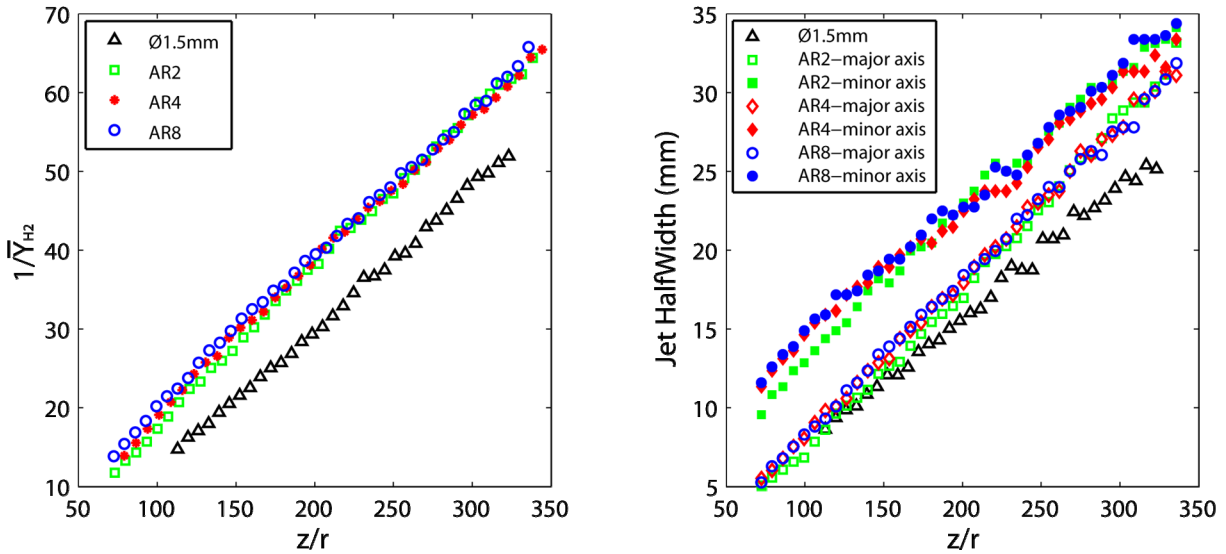
Figure 5. Left: Reciprocal mean mass fraction along the centreline with Jackknife uncertainties. Right: Jet half widths against normalized axial distance.
