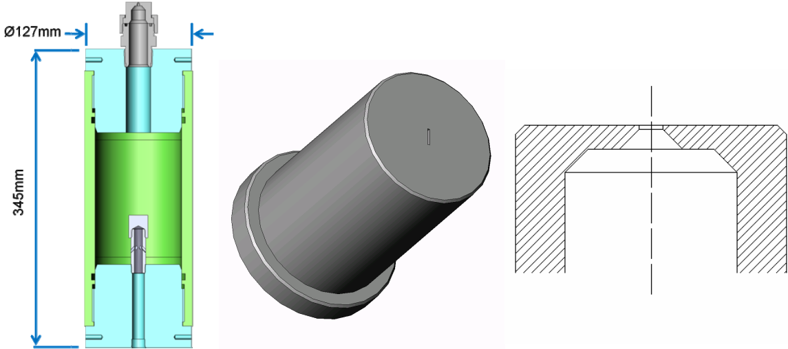
Figure 1. Sectional view of the stagnation chamber and nozzle assembly (left) along with a picture of the nozzle with the AR 8 exit (centre) and a corresponding sectional view (right).
