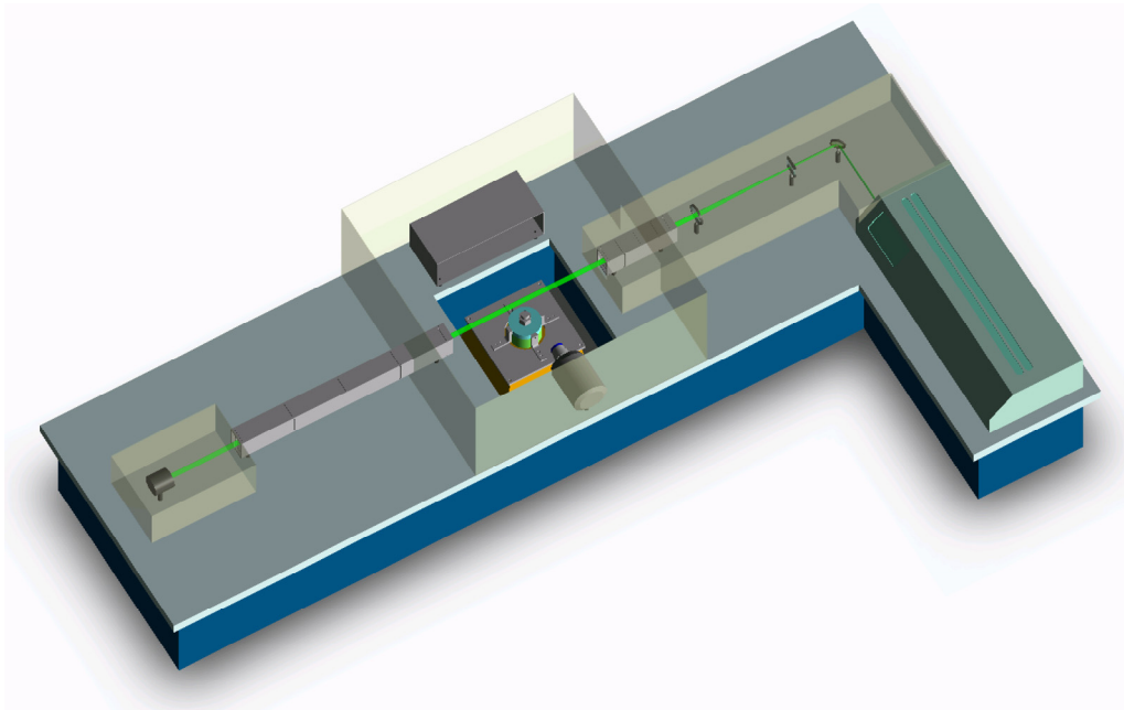
Figure 2. Detailed illustration of the planar Rayleigh laser scatter setup.
